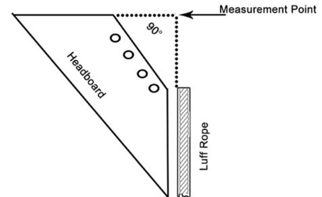
G.6.c. FORWARD UPPER CORNER OF HEADBOARD
